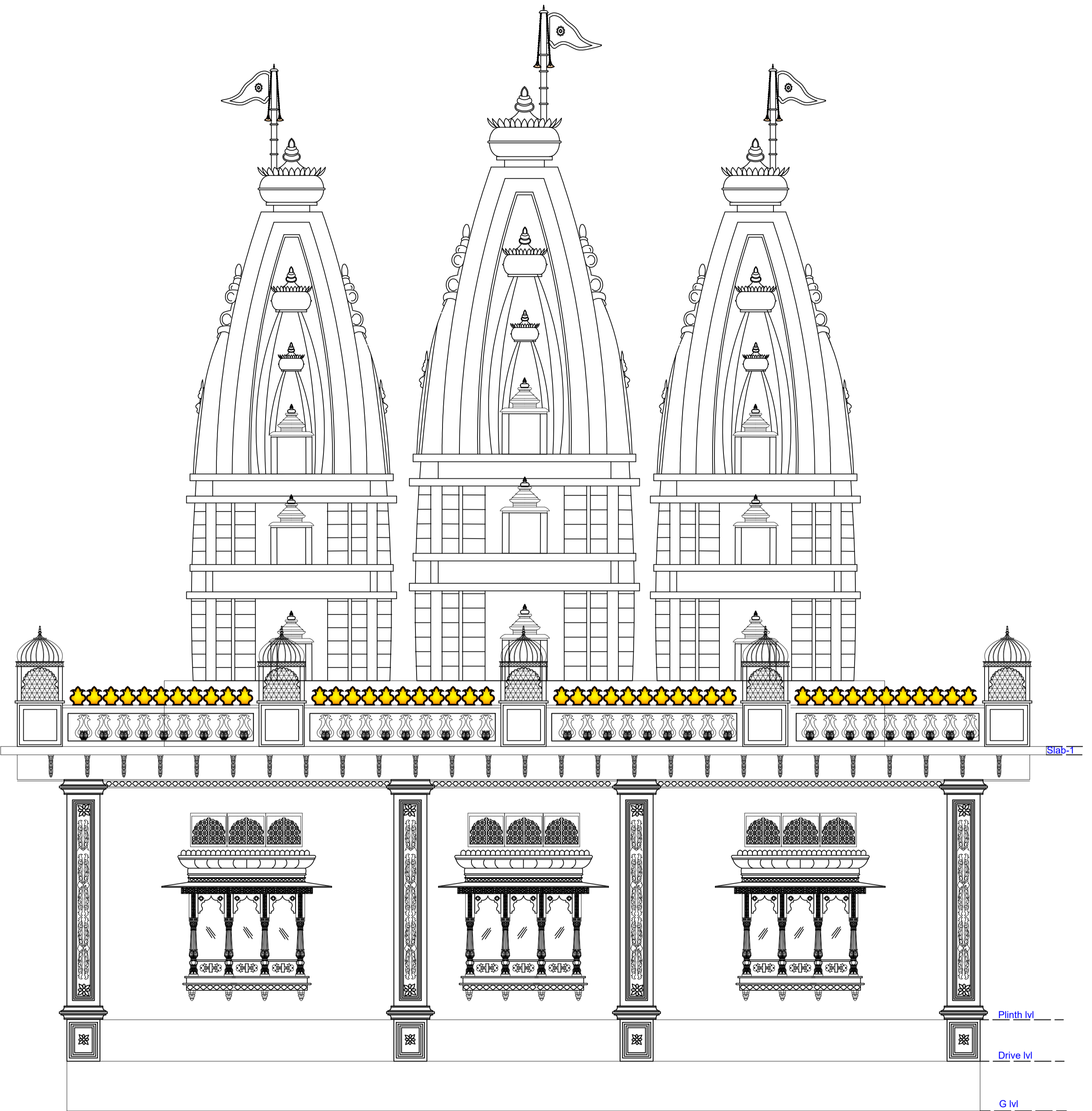
Back Side Elevation Details
